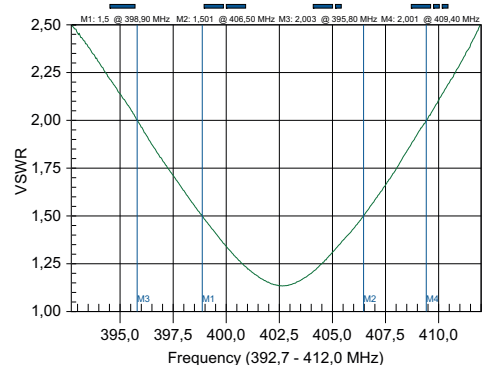
TYPICAL VSWR A-300MU-N
